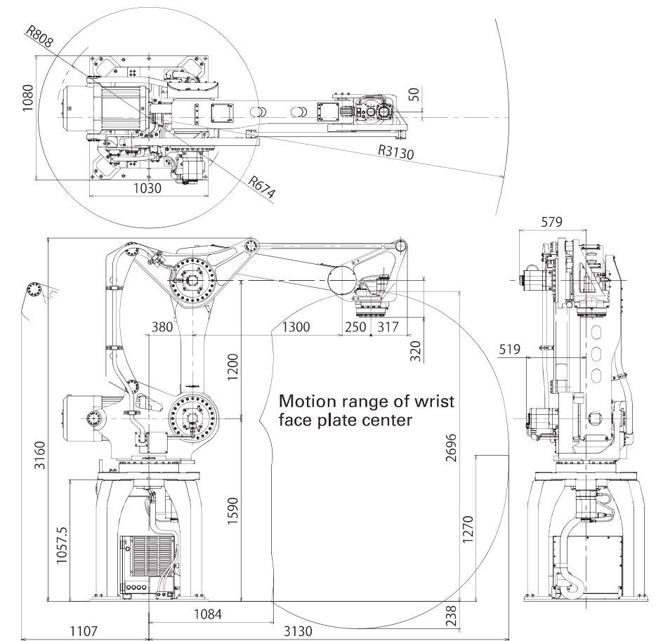
Operating space ( M-410iB/450 )
